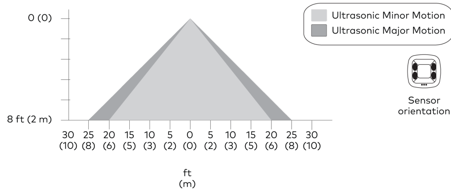
Side View Sensor Orientation A
