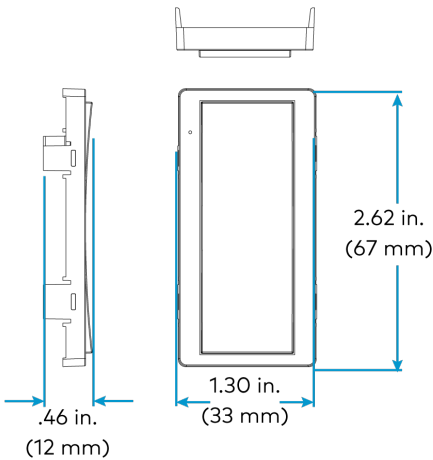
ZUMLINK-BTNR (BLANK shown)
