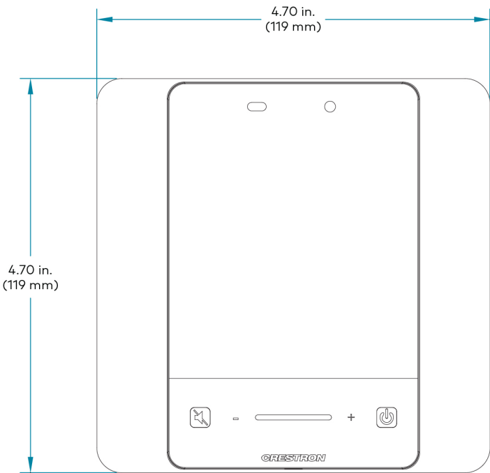
MPC3-101/102/201-RMB with MPC3-101-B or MPC3-102-B installed
