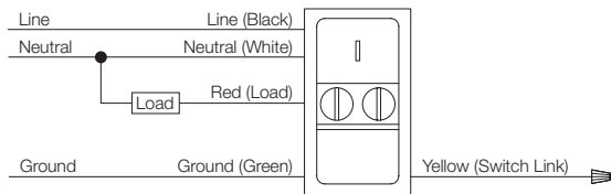
WLS 1 Basic Wiring
