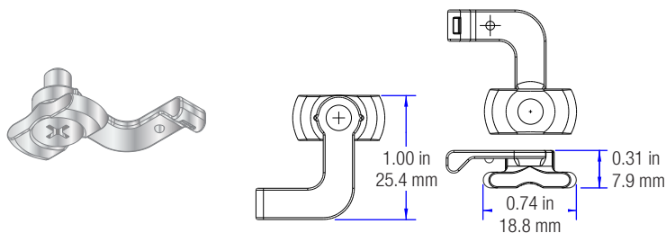
Cam Lock Mounting Bracket (Qty. 2) (CSA-DRP-CAM-LOCK)
