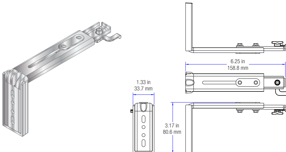
Mounting Bracket, Single (Qty. 2) (CSA-DRP-BRKT)
