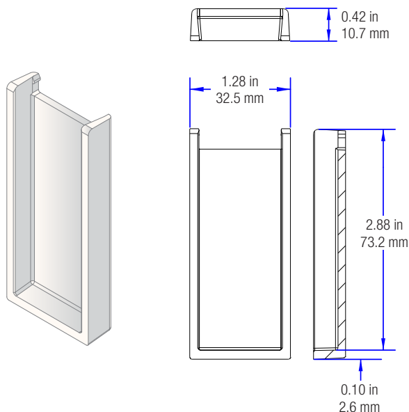
Bracket End Cap (Qty. 2) (CSA-DRP-BRKT-CAP)
