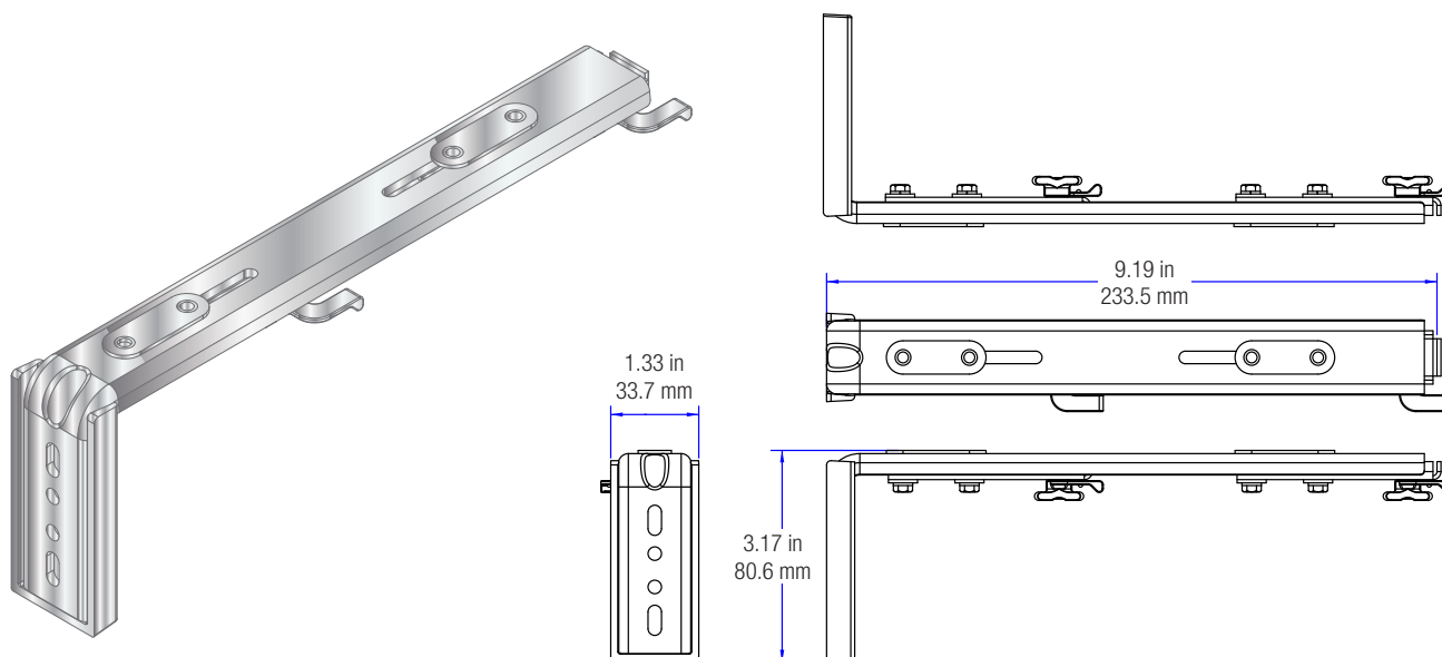
Mounting Bracket, Dual (Qty. 2) (CSA-DRP-BRKT-DUAL)
