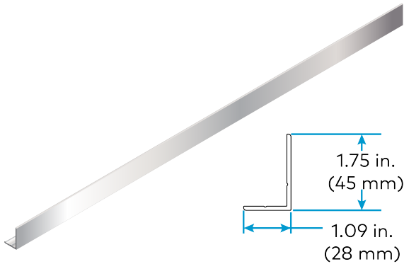
H-Channel (CSA-ARCH-BO-CHANNEL-H)
