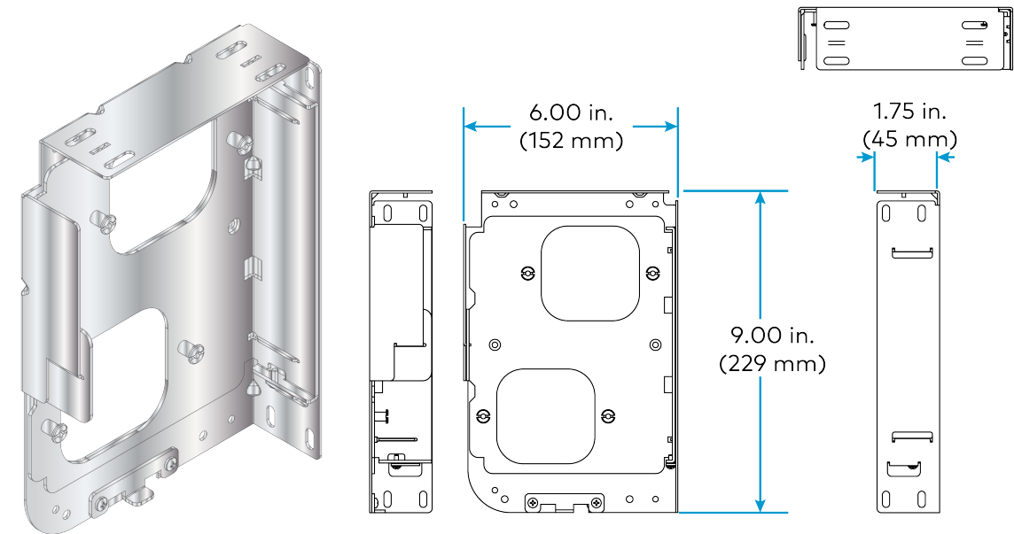
Dual Mounting Bracket, Idler Side (CSA-ARCH5-BRKT-DUAL)
