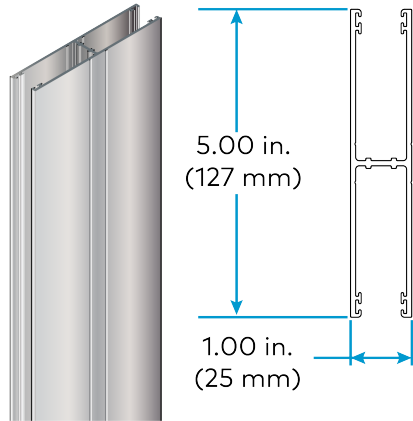
Channel Cap (CSA-ARCH-BO-CHANNEL-CAP)
