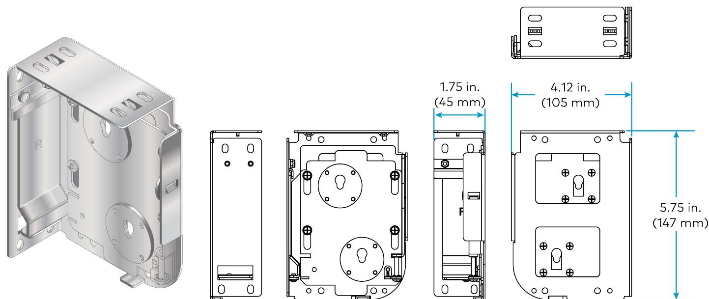
Dual Mounting Bracket, Idler Side (CSA-ARCH3-BRKT-DUAL)
