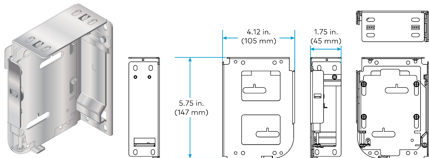
Dual Mounting Bracket, Idler Side (CSA-ARCH3-BRKT-DUAL)
