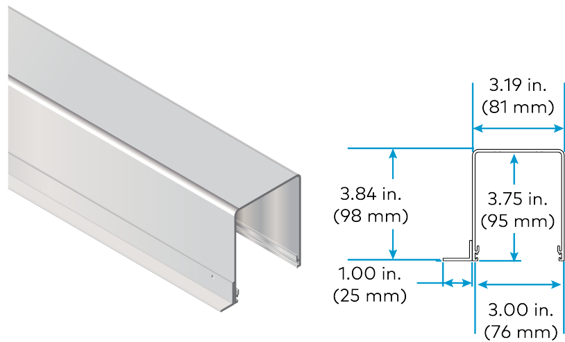
Pocket with Tile Lip
