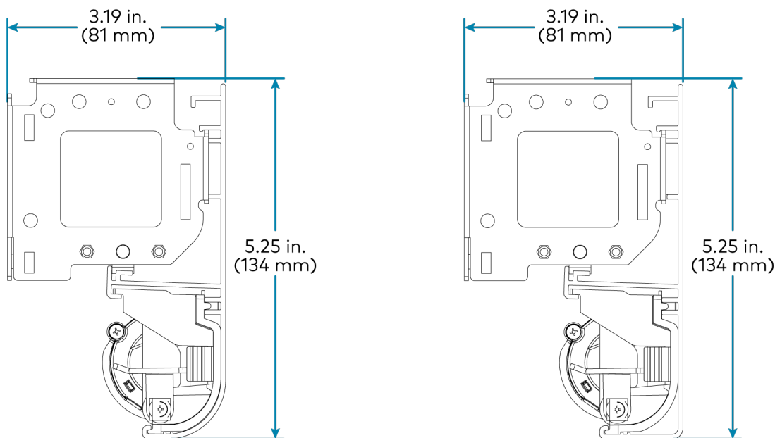
CSS-ARCH3 Dimensions with Fascia (Curved and Square)
