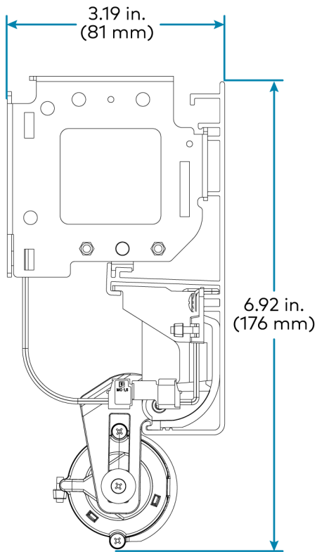
CSS-ARCH3 Fascia (Curved and Square)
