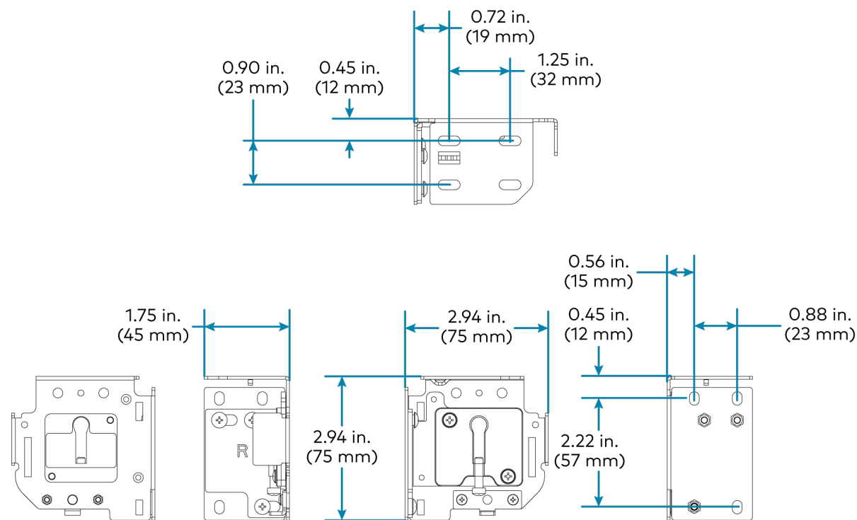
CSS-ARCH3 Dimensions with Fascia (Curved and Square)
