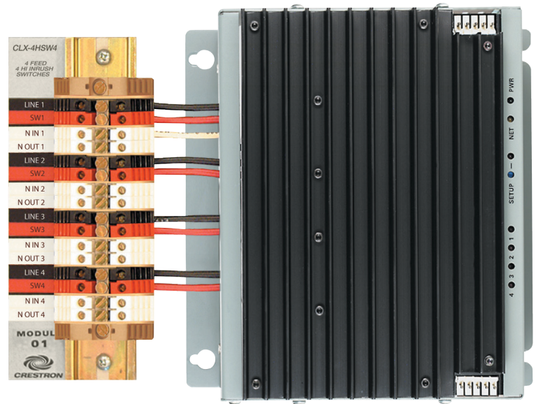
Shown with CLT-4HSW4 terminal block (sold separately)
