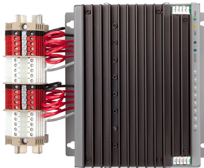
Shown with CLT-2DIMU8-277 terminal block (sold separately)
