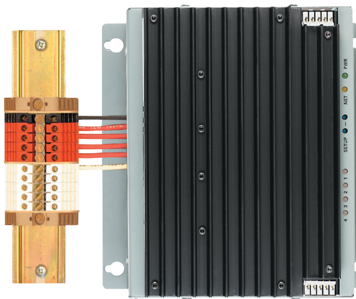
Shown with CLT-1DIMU4 terminal block (sold separately)
