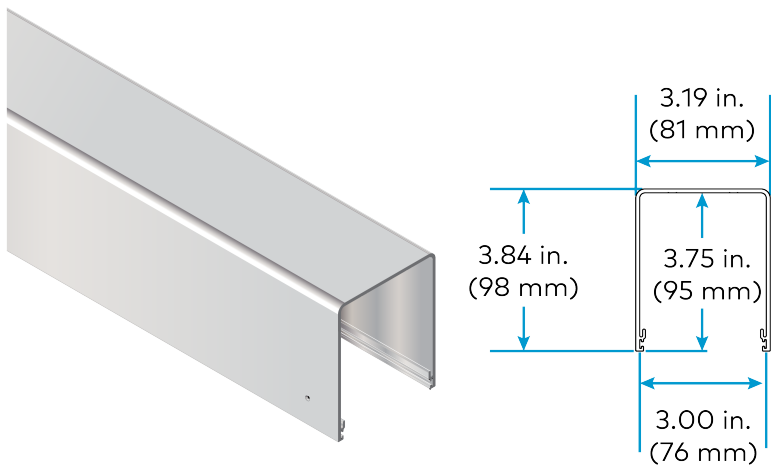
Pocket with Tile Lip
