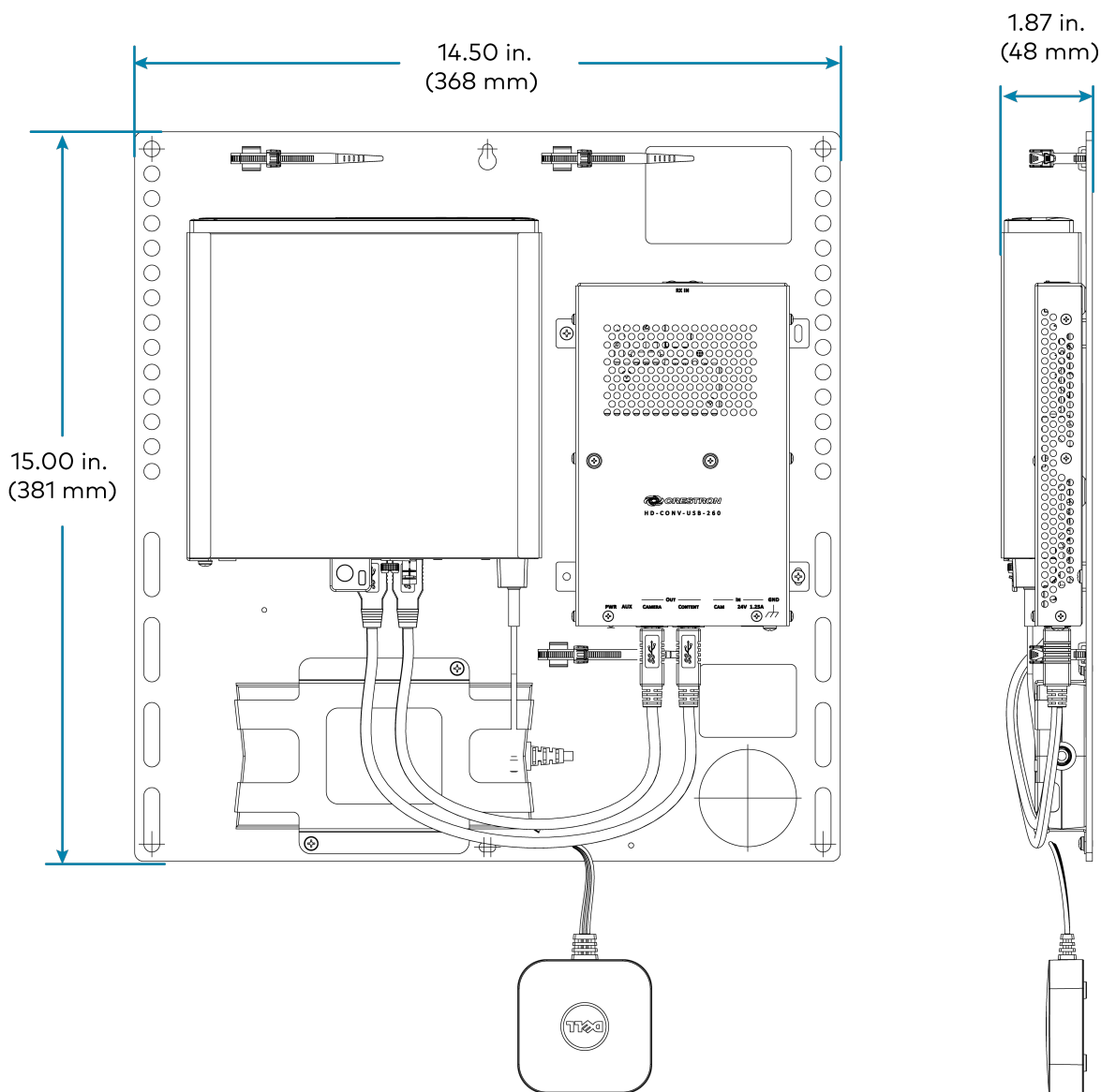
UC Bracket Assembly (UC-BRKT-260-PRO-Z-ASSY)
