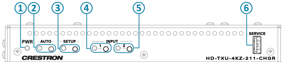
HD-TXU-4KZ-211-CHGR Transmitter, Front Panel
