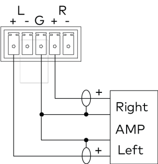
Unbalanced Output
