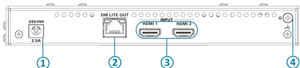
HD-TX-4KZ-201 Rear Panel
