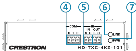
HD-TXC-4KZ-101 Front Panel
