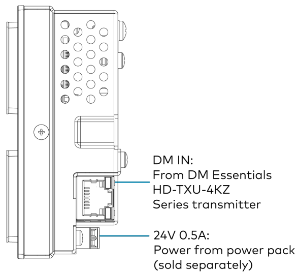
HD-RXU-4KZ-101-2G Rear, Top View
