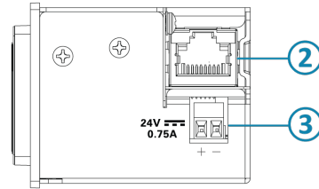
1G Wall Plate Transmitter, Rear, Top View
