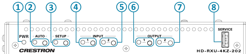
HD-RXU-4KZ-202 Receiver, Front Panel
