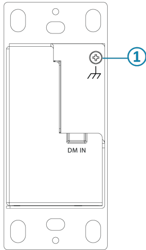
1G Wall Plate Receiver, Rear
