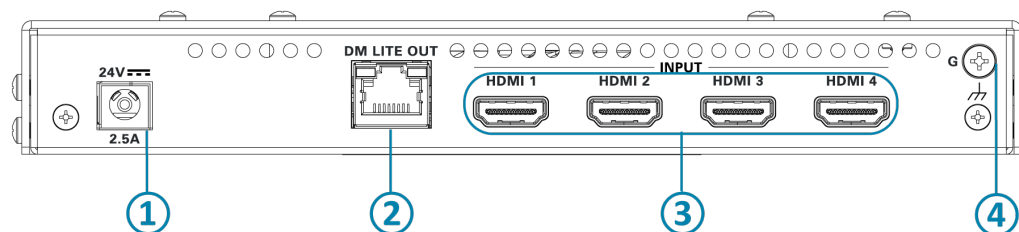
HD-TX-4KZ-401 Rear Panel
