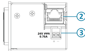
1G Wall Plate Receiver, Rear, Top View
