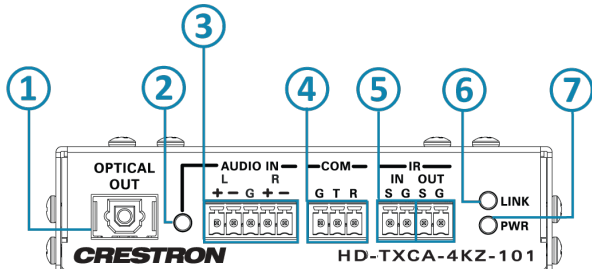
HD-TXCA-4KZ-101 Front Panel
