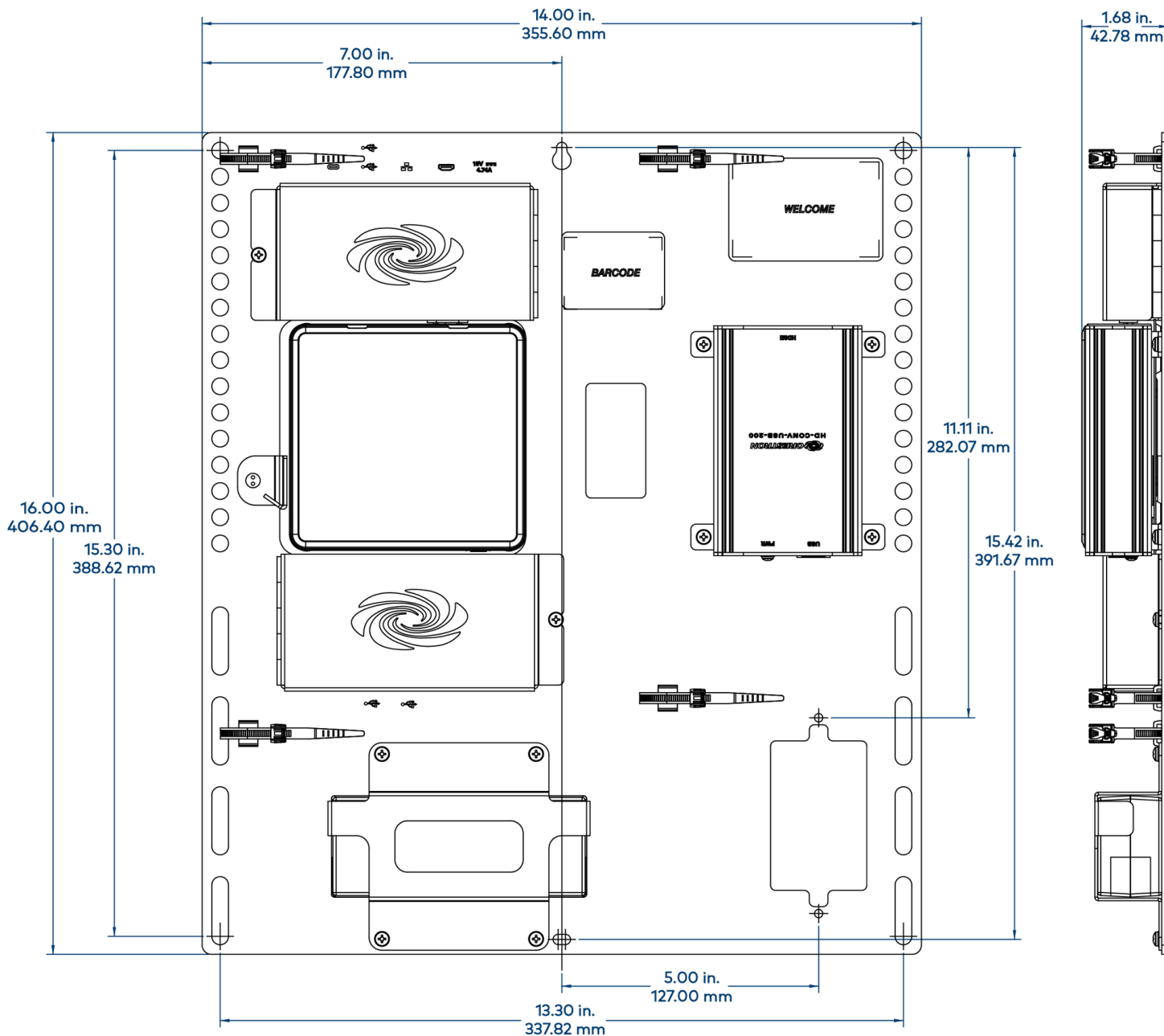
UC-BRKT-100-SD-ASSY
