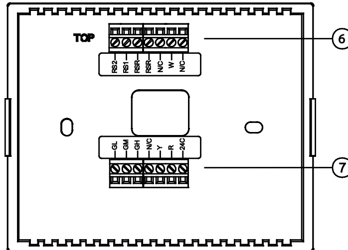
CHV-TSTATEX-FCU (Connection View, Front with Cover Removed)
