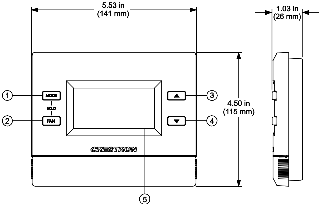
CHV-TSTATEX-FCU Overall Dimensions (Front and Side Views)
